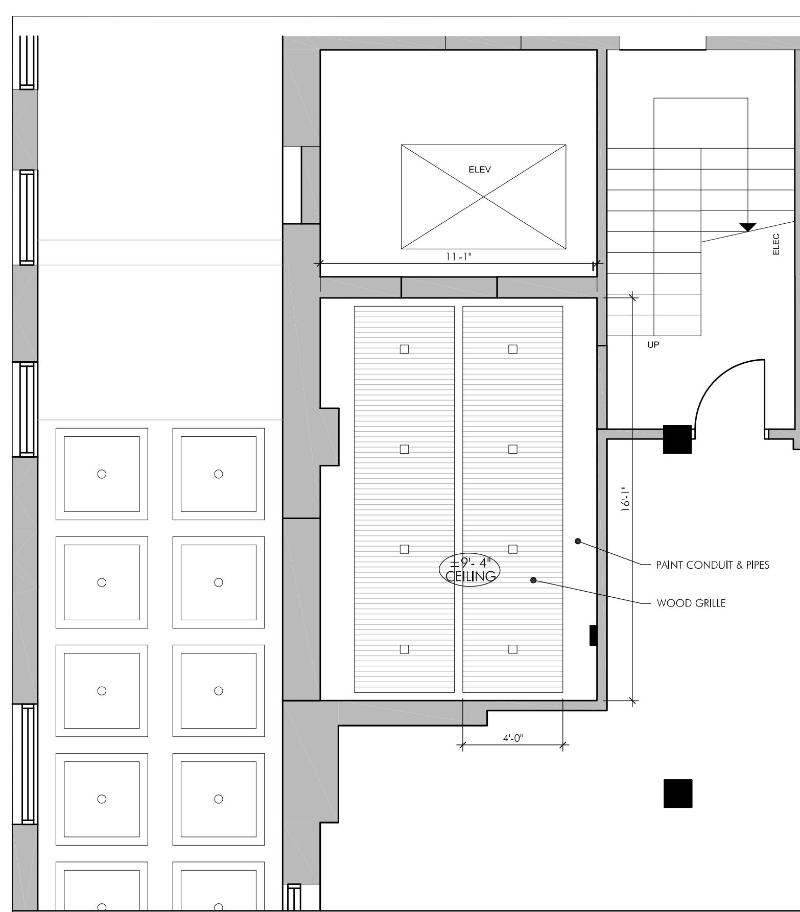
1 PROPOSED CEILING PLAN SK1 SCALE: 1/4" = 1'-0"
